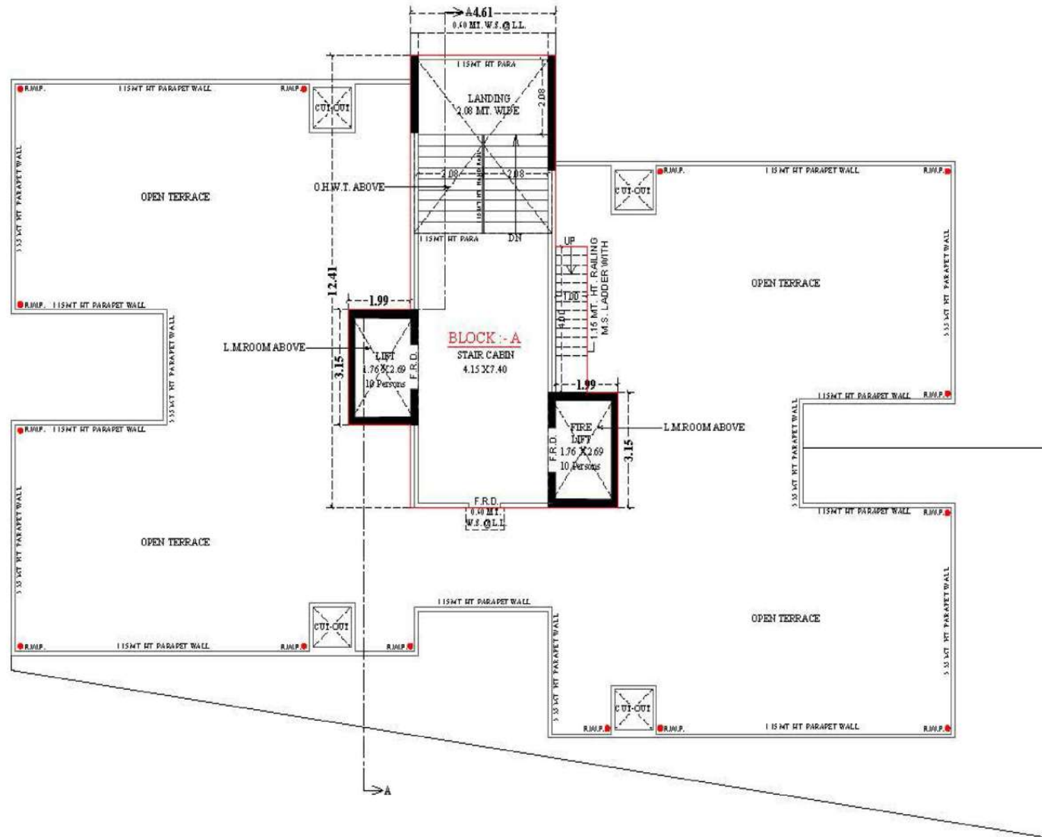
OPEN TERRACE PLAN WITH (STAIR CABIN, LIFT MACH.ROOM&O.H.W.T.)
