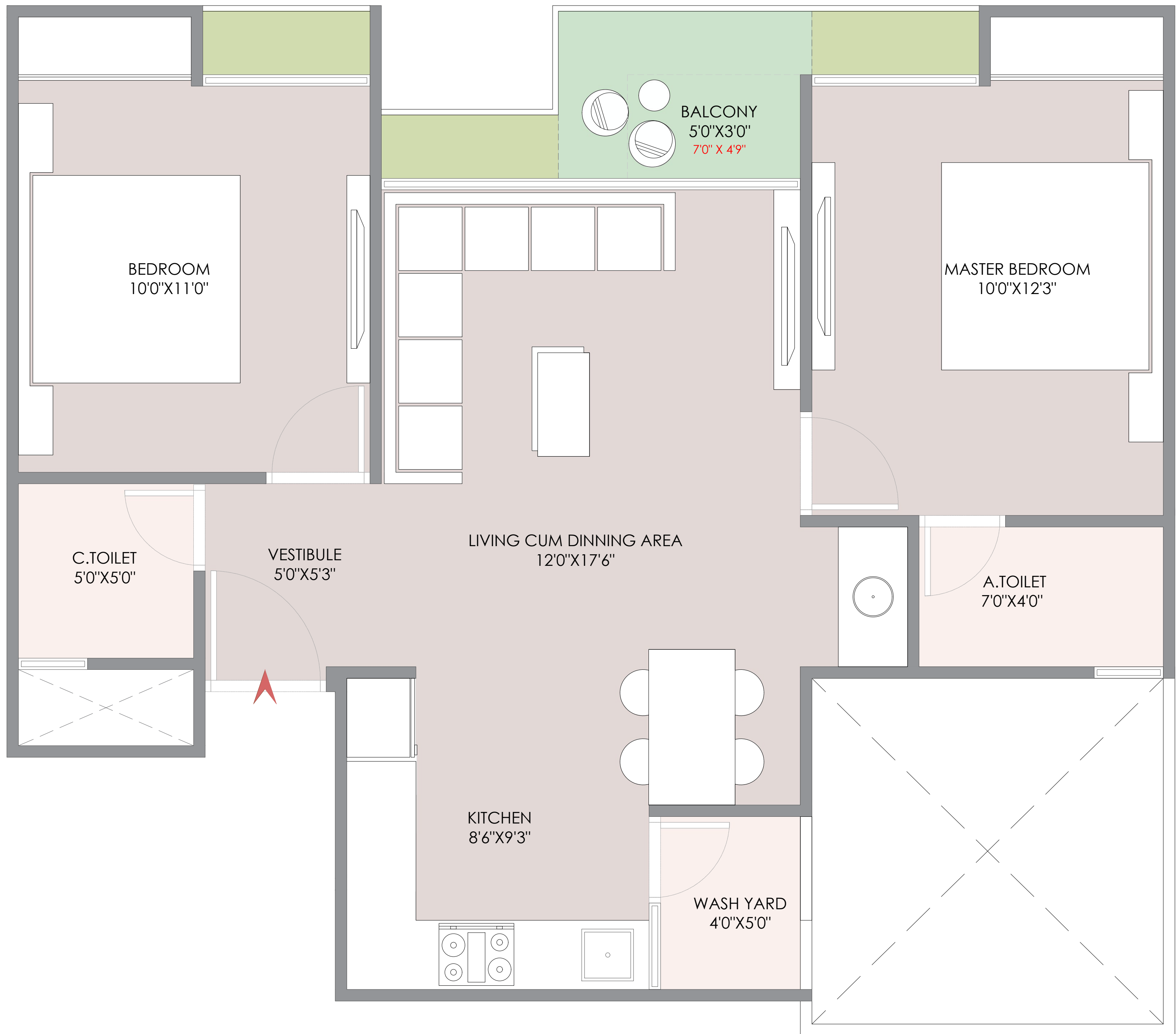
PROPOSED UNIT LAYOUT TYPE 04
