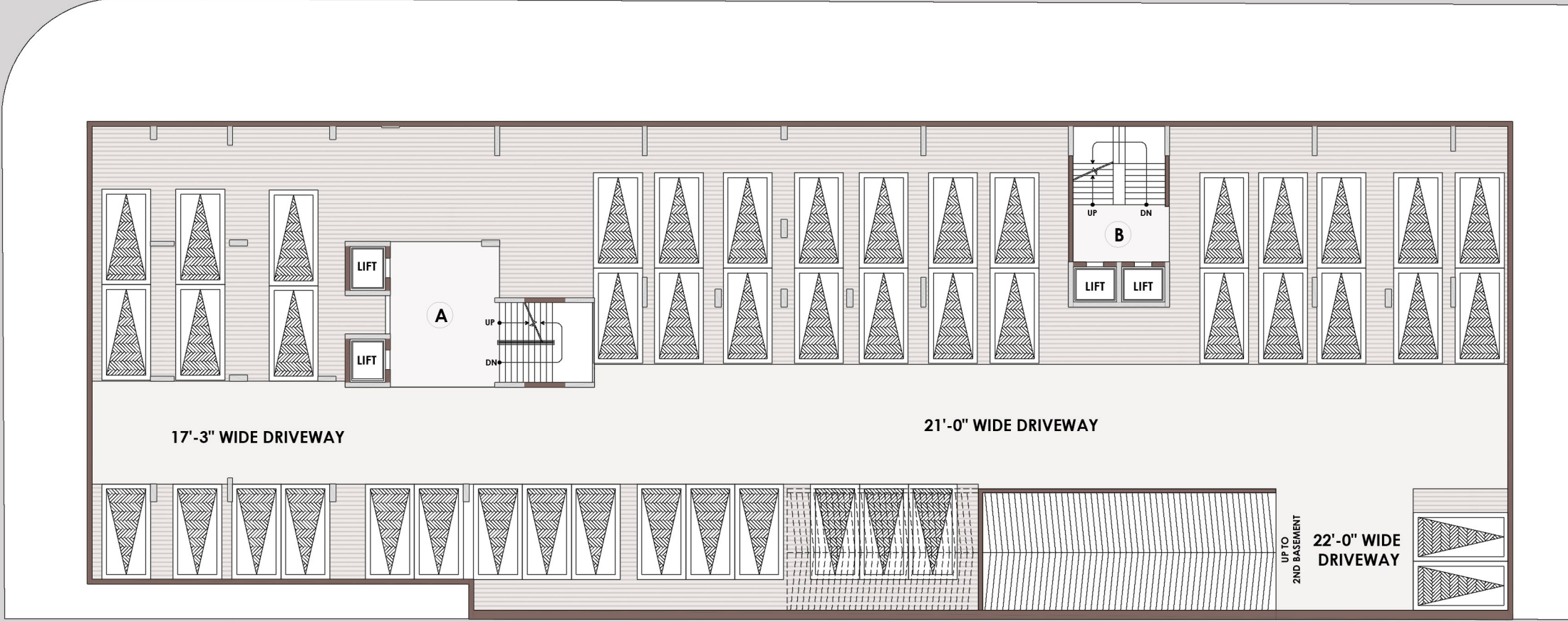
BASEMENT -3 PLAN
