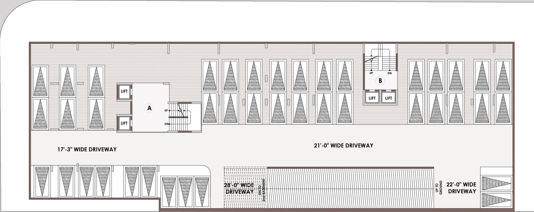
BASEMENT -1 PLAN
