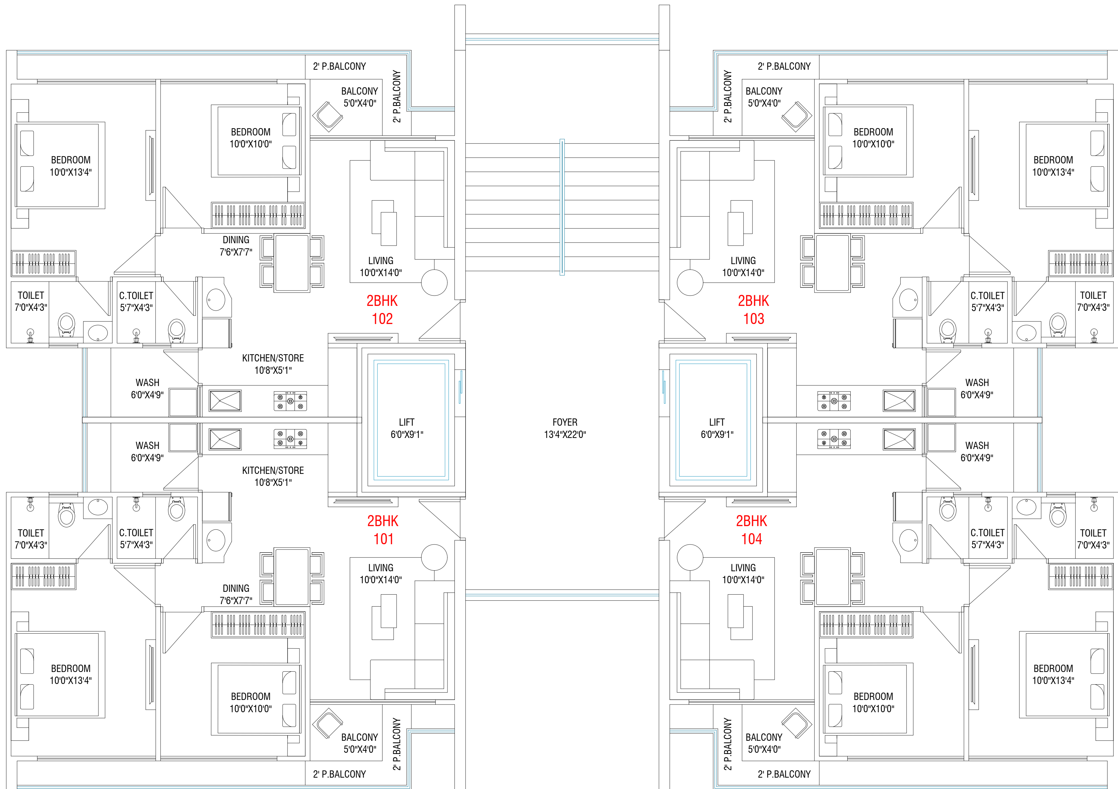
2BHK TYPICAL FLOOR CLUSTER PLAN D & E
